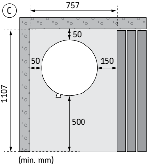
Figure 6. Safety distances
