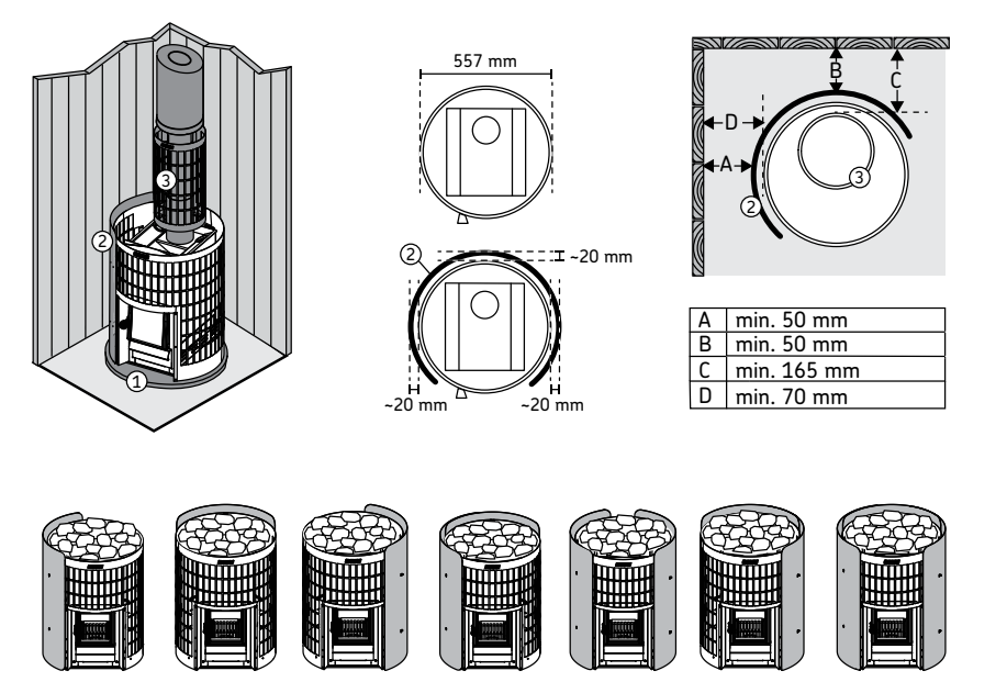
Figure 8. Protective accessories (dimensions in mm)
